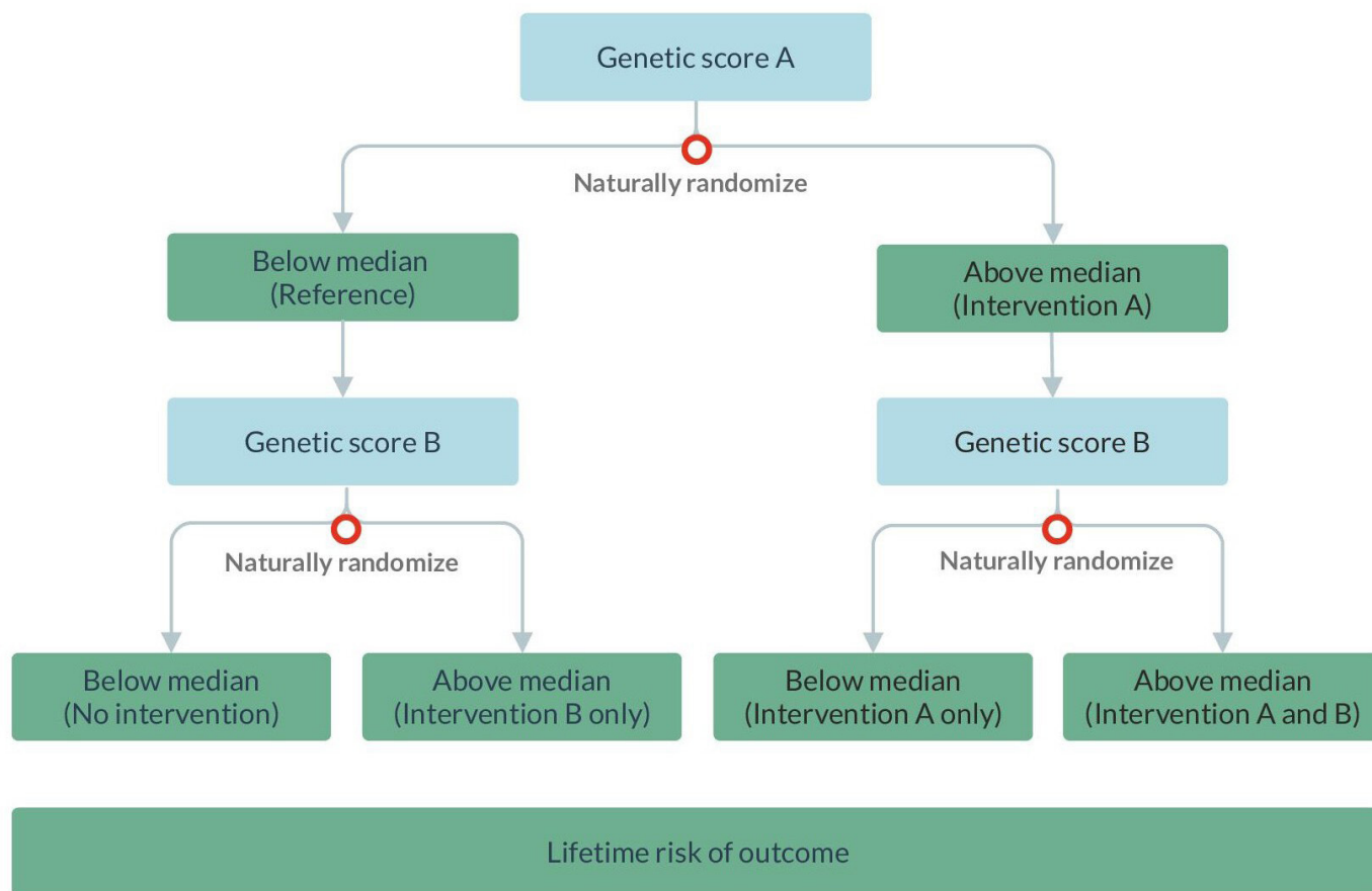
Figure 3 Schematic diagram illustrating a 2x2 factorial Mendelian randomisation design with dichotomised genetic risk scores that acts proxies for interventions on exposures A and exposure B.
